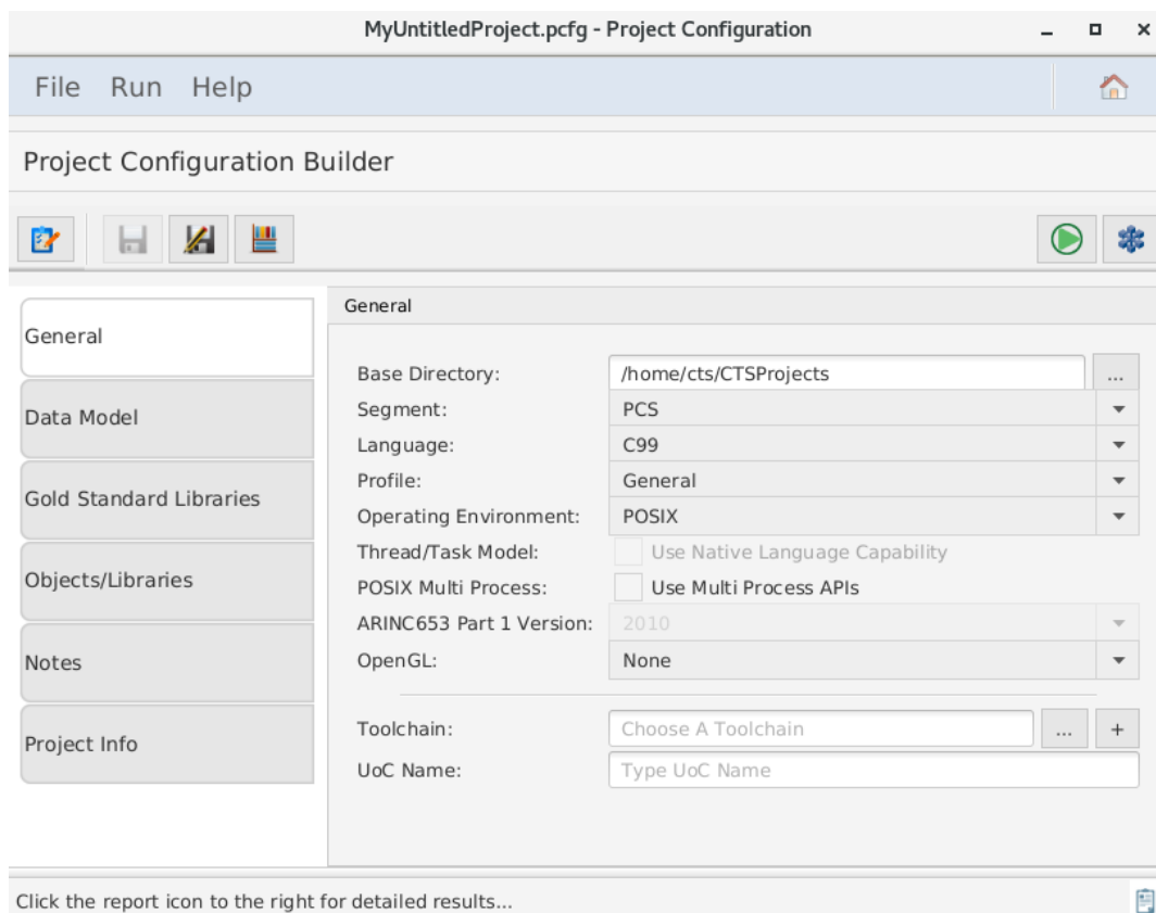
Figure 28. The Project Configuration Builder with the General tab selected.
