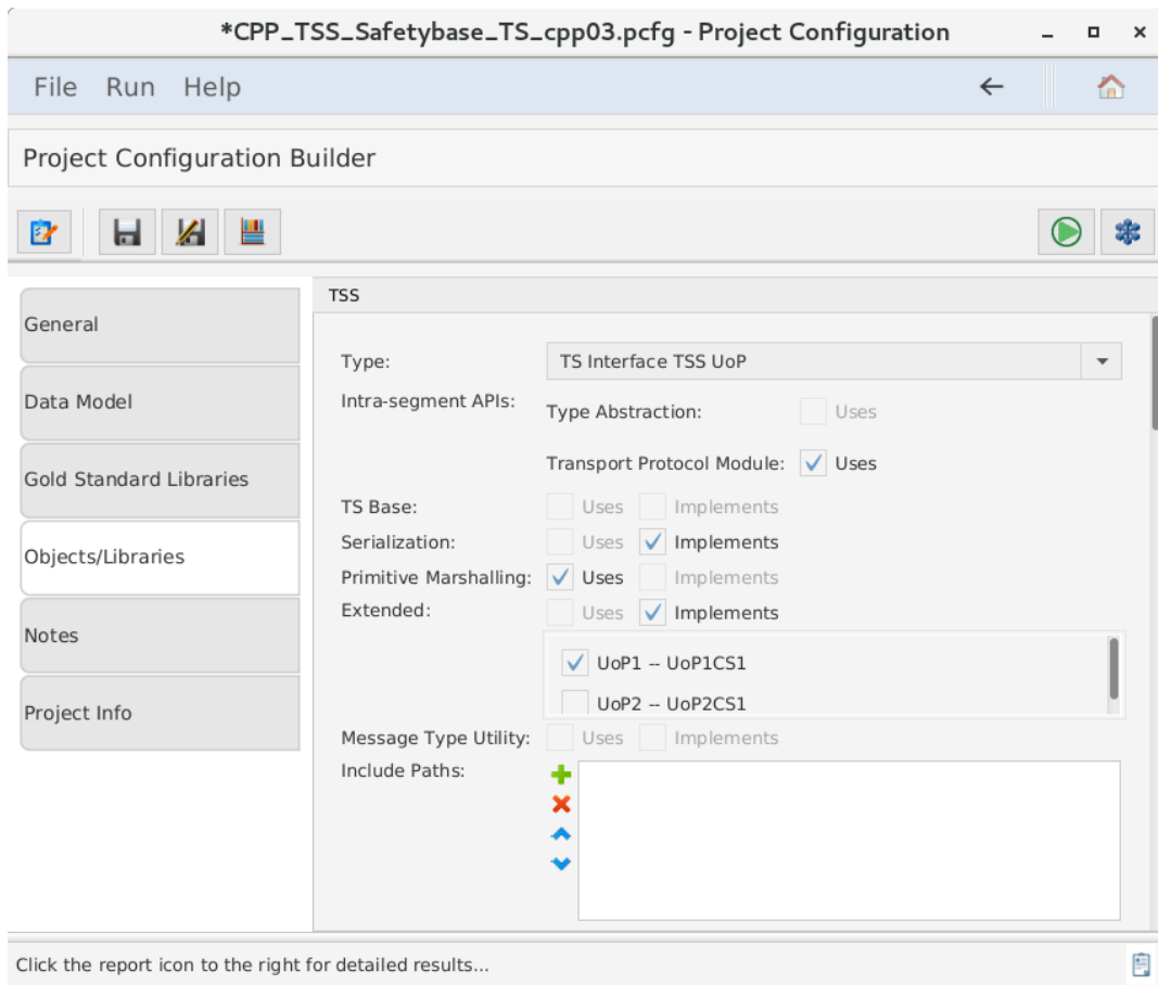
Figure 66. Include Paths and Files
